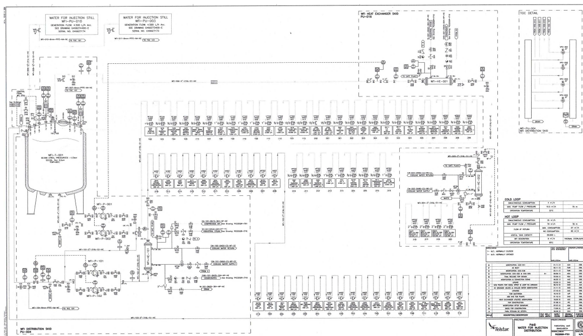
Fig. 1. A sample WFI distribution diagram for a large volume parenteral production unit
