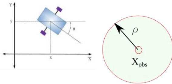
Fig. 2: Unicycle-like robot with obstacle avoidance region
