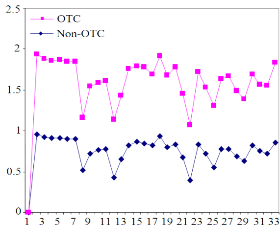
Fig. 9: Efficiency on different programs (OTC Vs non OTC)
