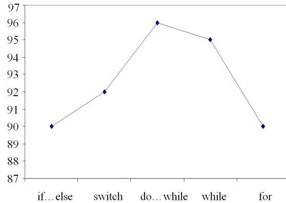
Fig. 7: Percentage Efficiency in code conversion for control structures
