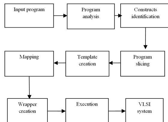
Fig. 2 RL2M Architecture Diagram
