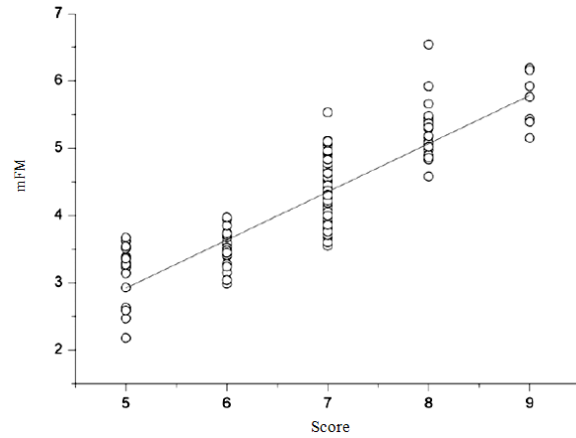
Fig. 11: Graphic illustration of the correlation observed between the measurements provided by the cavitometer and the cleaning test
